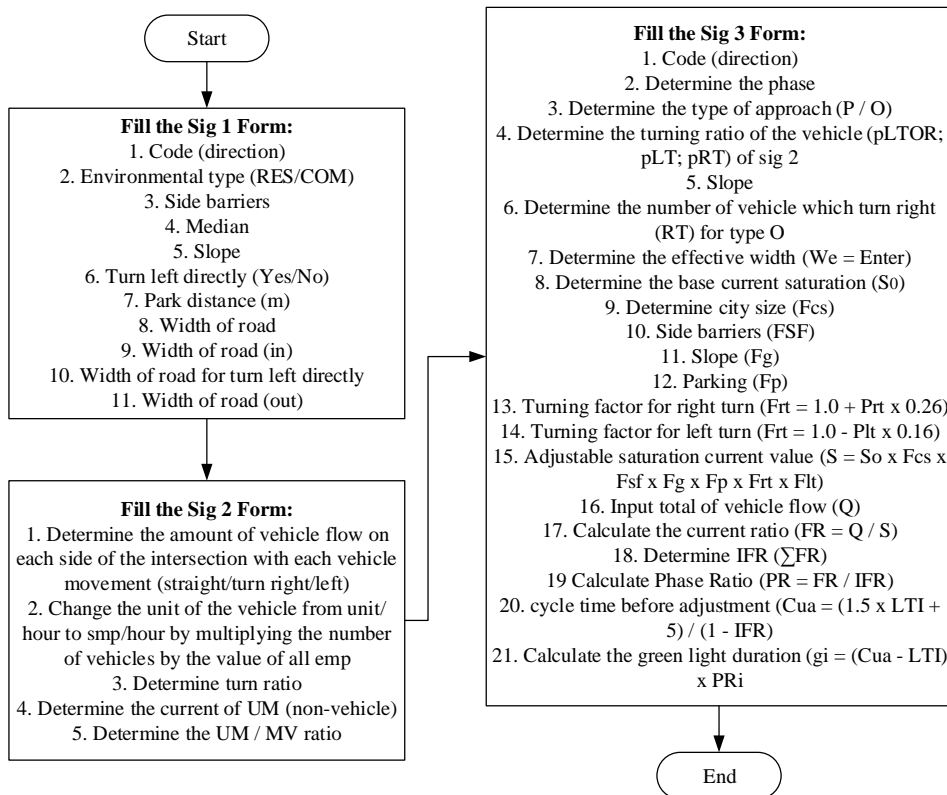
Fig. 4 – The Procedure of MKJI in Calculating The Green Duration
