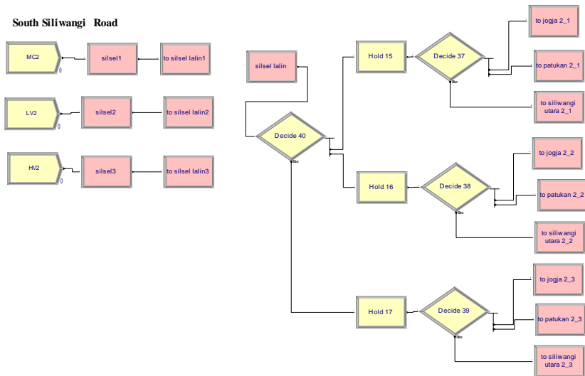
Fig. 9 – The current simulation model (South Siliwangi Road)
